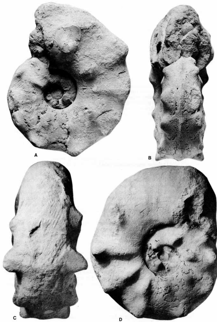
TEXT-FIG. 9. Lecointriceras fleuriausianum (d'Orbigny) A, B. EMP A35.3, 'Bassin de la Loire, achète de Stur' — the original of d'Orbigny's (1841) pl. 108, fig. 2. Reduced \times 0.66 . C, D. FSM 119, an adult from Poncé, Sarthe(?) showing the smooth, tubular termination to the body chamber. Reduced \times 0.6 approx.
