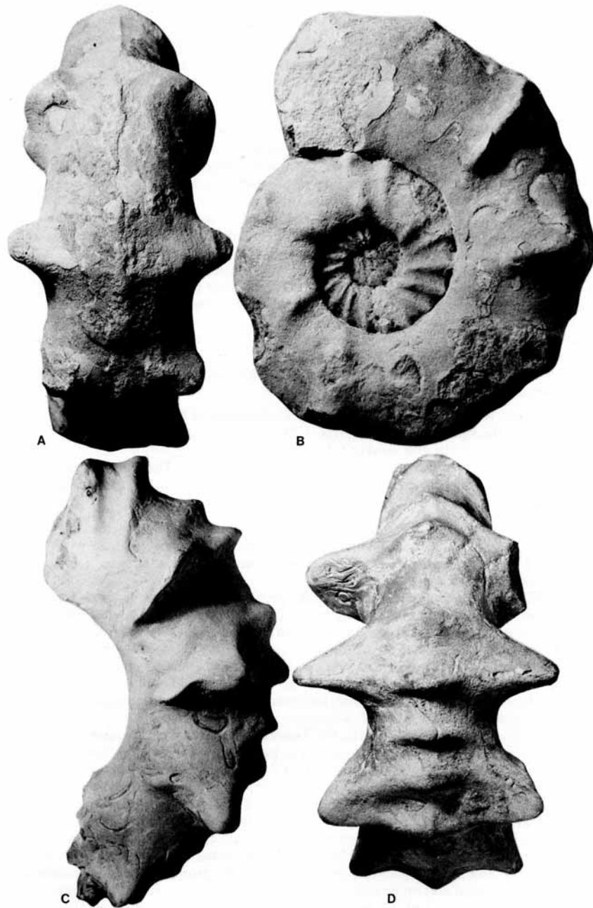
TEXT-FIG. 3. Collignoniceras woollgari (Mantell) A, B, MNHP W14, 6778 (d'Orbigny Collection), from Poncé, Sarthe. A. tuffeau specimen agreeing closely with the type. Reduced \times 0.5 approx. C, D. MNHP 1946-19, from St. Maure de Touraine. A hypernodose adult of the first type. Reduced \times 0.4 approx.
