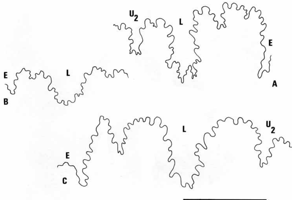
TEXT-FIG. 1. Sutures of Collignoniceras species. A, C. woollgari (Mantell), from BMNH C74803; B, C. carolinum (d'Orbigny), from the Sorbonne specimen (de Grossouvre Collection); C, C. papale (d'Orbigny), from a Sorbonne specimen (de Grossouvre Collection). Bar scale is 2 cm.
