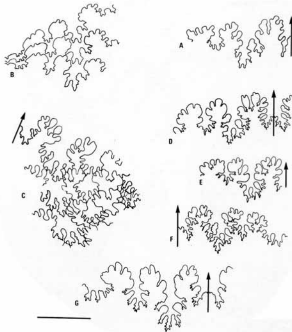
TEXT-FIG. 2. A-G, Neptychites cephalotus (Courtiller). Sutures of: A: the missing paralectotype (after Pervinquière 1903a, fig. T5; B: typical Tunisian example (after Pervinquière 1907, fig. 152); C: N. gourguechoni (after Pervinquière 1907, fig. 156); D: N. telingaeformis (after Solger 1904, fig. 11b); E: N. telingaeformis palmata (after Solger 1904, fig. 16); F: N. telingaeformis elegans (after Solger 1904, fig. 15); G: N. crassus (after Solger 1904, fig. 18). Bar scale is 2 cms.
