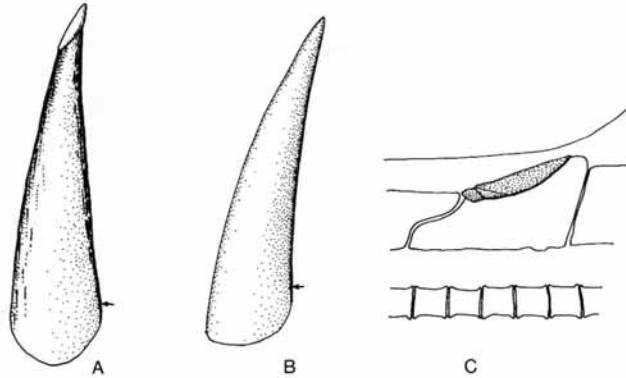
TEXT-FIG. 4. Various rhinobatid fin spines (not to scale). A, Belemnobatis annectans (from B.S.P.H.G. 1963-1-19, Munich). B, Belemnobatis sismondiae (from Pi 1210/13, Tübingen). C, Spathobatis bugesiacus (from BM (N.H.) P.2099).
