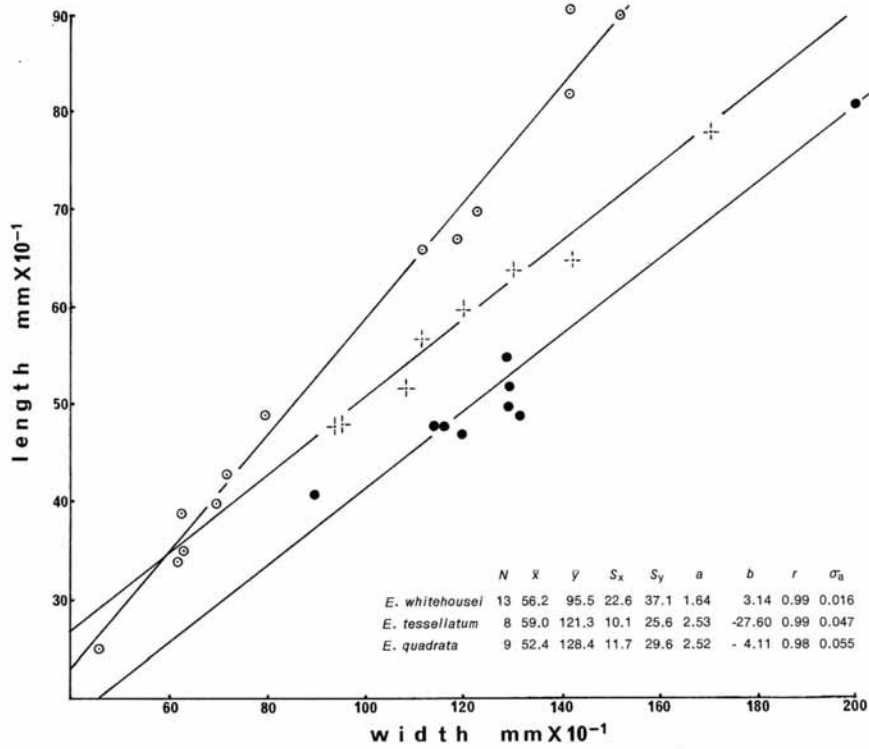
TEXT-FIG. 3. Reduced major axis regressions of pygidial width plotted against pygidial length for Idamean species of Eugeonocare . Symbols for tabulated statistics are as for text-fig. 2.
