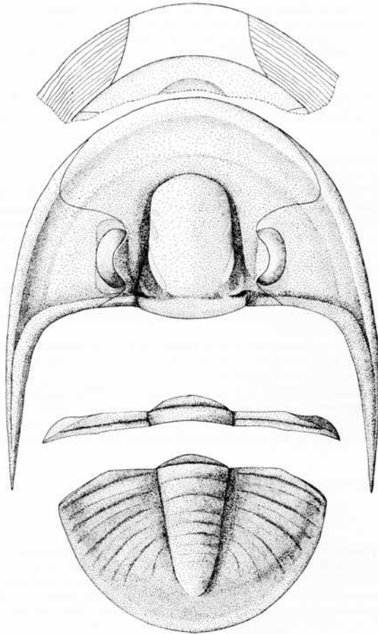
TEXT-FIG. 1. Reconstruction of Radnoria syrphetodes gen. et sp. nov. Topmost illustration represents the ventral aspect of the anterior part of the cephalon to show the inferred shape of the rostral plate (blank area). All \times 11 approx.
