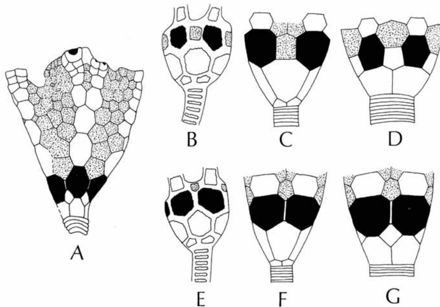
TEXT-FIG. 3. Origin of Dimerocrinites pentlandicus sp. nov. A, lateral view of holotype; note shape of primibrachs, structure of interbrachials, and zygodiplobathrid base, \times 3\text{--}4 . B-D, sketches showing probable ontogeny of rhodocrinitids with eudiplobathrid base and zygodiplobathrids. B, 'larva' of dicyclic camerate crinoid with interbrachials separating the radials; note that the plates are still separated by tissues; during later ontogeny, these join to form a rigid mosaic of plates; reconstructed by analogy with living crinoids, based on the growth sequence of plates and statistical data of Brower (1973, pp. 292-328); height of larval calyx is about 0.5 mm. C, D, bases of mature crinoids simulated by growth of the 'larva'. C, eudiplobathrid base of rhodocrinitid, growth rates of height and width of the plates relative to total size of the calyx: infrabasals 0.14, basals 0.43, radials 0.43. D, zygodiplobathrid base, relative growth rates of height and width of the plates: infrabasals 0.62, basals 0.13, radials 0.25. E-G, sketches showing postulated ontogeny of zygodiplobathrid base seen in D. pentlandicus sp. nov. and normal dimerocrinitids. E, 'larva' of dicyclic camerate crinoid in which the proximal interbrachials are at the level of the primibrachs, reconstructed as before. F, G, bases of mature dimerocrinitids simulated by growth of the 'larva'. F, eudiplobathrid base of normal dimerocrinitid, relative growth rates for plates: infrabasals 0.14, basals 0.43, radials 0.43. G, zygodiplobathrid base of D. pentlandicus sp. nov., relative growth rates for plates: infrabasals 0.62, basals 0.13, radials 0.25. All relative growth rates of plates are approximate averages for both height and width. Symbols: radials black, interbrachials stippled.
