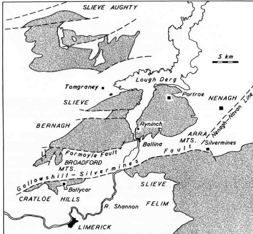
TEXT-FIG. 1. Locality map of the Limerick area. Lower Palaeozoic inliers shaded. Broken lines, faults; complete lines, stratigraphical contacts. Fossil localities of Ballycar (Cratloe Hills) and Ryninch (Arra Mountains) indicated.
