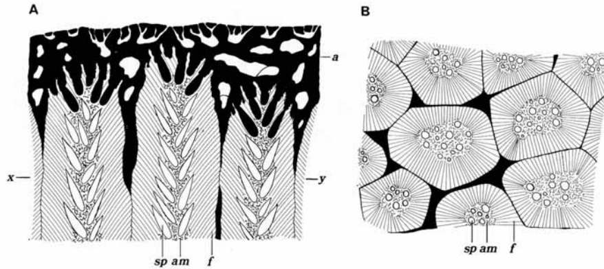
TEXT-FIG. 1. Murania lefeldi gen. et sp. nov. Diagrammatic details of the skeleton structure in (A) longitudinal and (B) transverse section, \times 50 .
