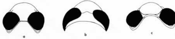
TEXT-FIG. 3. Outline reconstructions to show similarity of anterior cephalic profiles of Opipeuter , Pricyclopyge , and Carolinites . Visual surfaces black. a, Opipeuter inconnivus gen. et sp. nov. (about \times 4 ); b, Pricyclopyge binodosa (Salter), after Marek (1961, text-fig. 8) ( \times 2 ); c, Carolinites sibiricus Chugaeva, based on new material of this species from the upper part of the Valhallfonna Formation, Ny Friesland, Spitsbergen ( \times 4 ).
