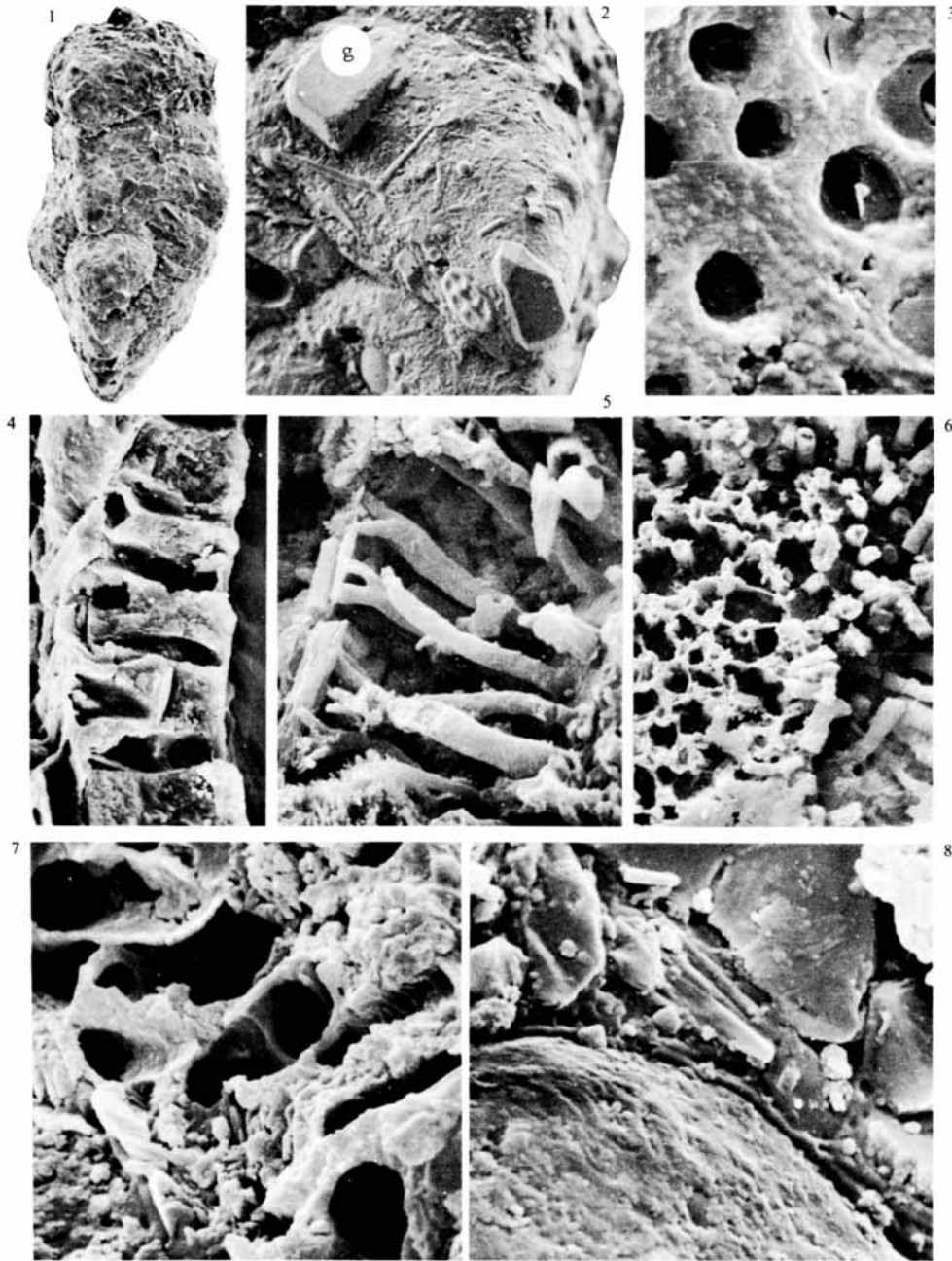
MURRAY, agglutinated foraminifera
