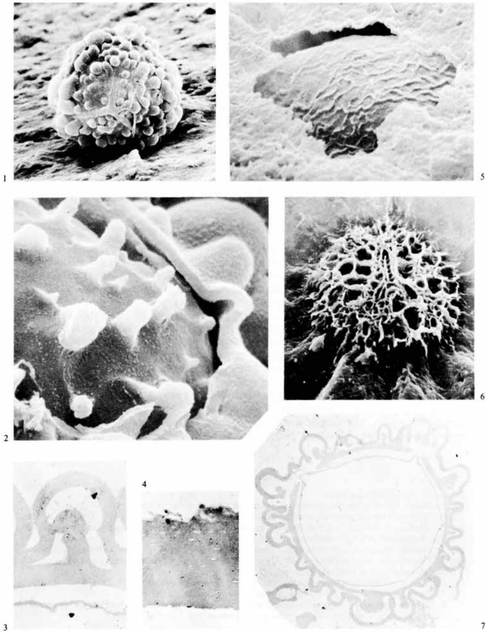
TAYLOR, Palaeozoic spores
