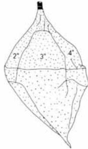
TEXT-FIG. 6. Diconodinium firmum sp. nov. Semidiagrammatic sketch of the holotype. × c. 1000.
