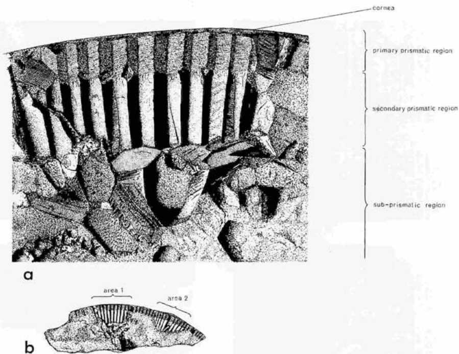
TEXT-FIG. 2. Drawings made from fracture surface of Gr 1 5508 showing areas of primary and secondary (diagenetic) calcite. a . Enlargement of area 1 \times 120 . b . Fragment of eye showing the two areas of secondary prisms, one of which is enlarged in a . \times 18 .
