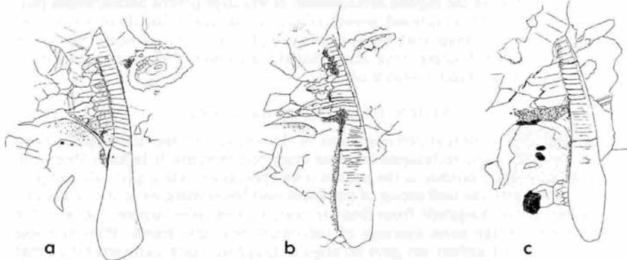
TEXT-FIG. 3. Effects of diagenesis shown in thin sections and cellulose peels of Gr I 5502. a . Oblique vertical section near posterior margin stained with methylene blue, showing primary and secondary prisms. b . Similar section, stained with alizarine red-S and acid fuchsine, with very irregular secondary prisms. c . Thin section through the same area, showing complete recrystallization of the secondary and partial alteration of the primary prisms. All \times 20 .
