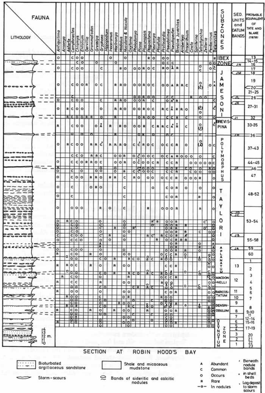
TEXT-FIG. 8. Stratigraphic section and faunal distributions at Robin Hood's Bay, Yorkshire.
