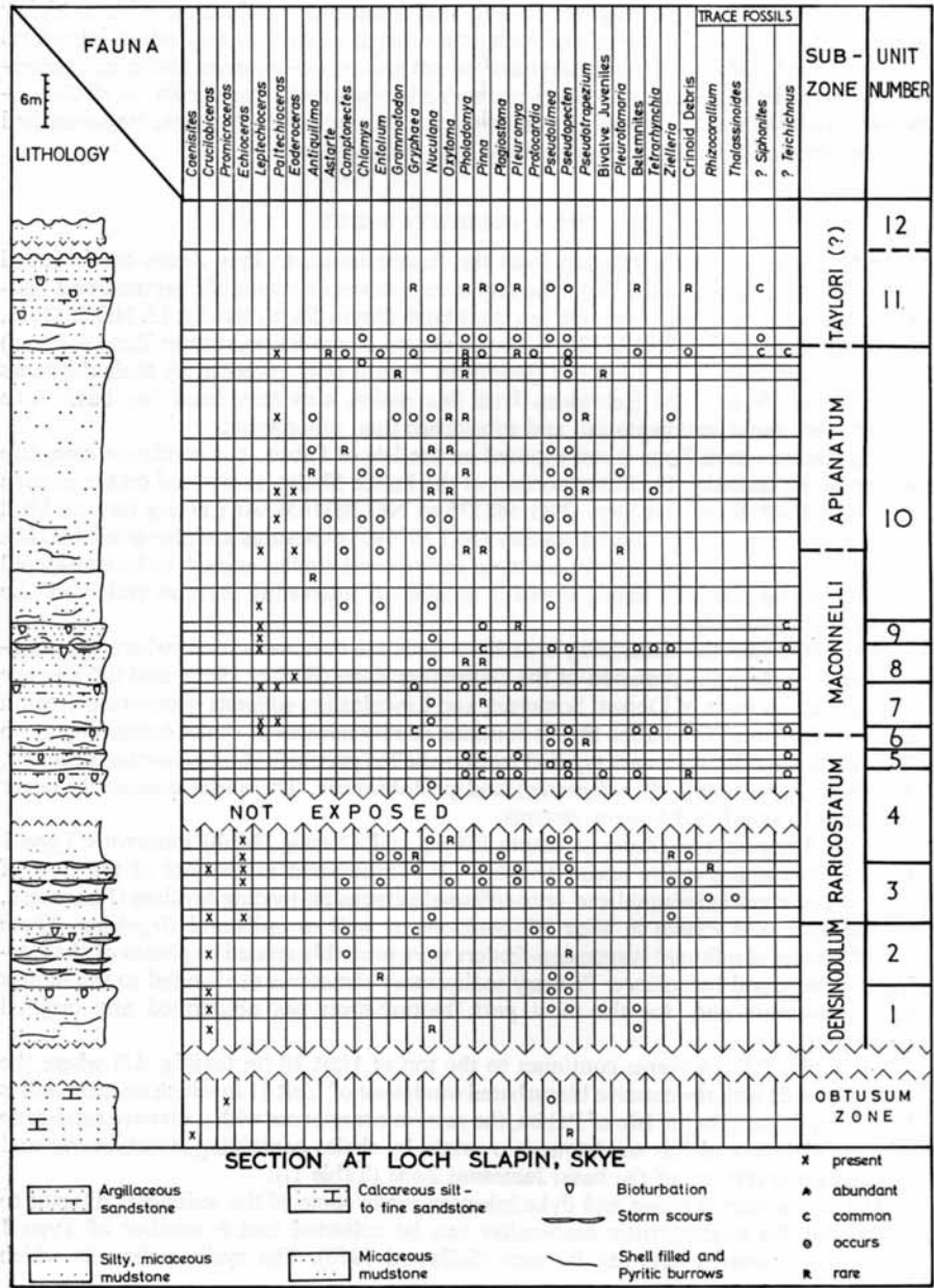
TEXT-FIG. 13. Stratigraphic section and faunal distributions at Loch Slapin, Skye.
