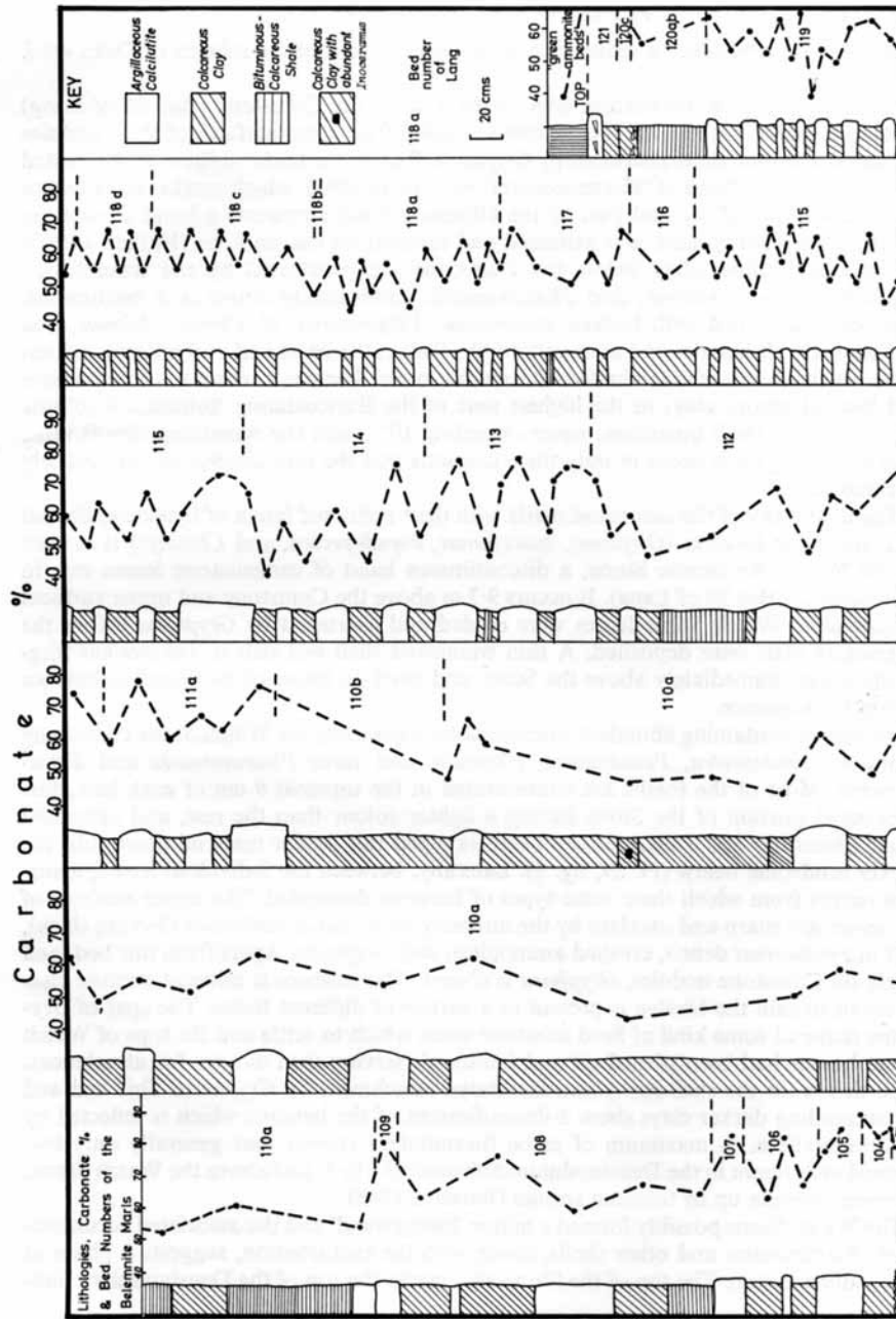
TEXT-FIG. 12. Stratigraphic sequence in the Belemnite Marls with insoluble residue data for each bed.
