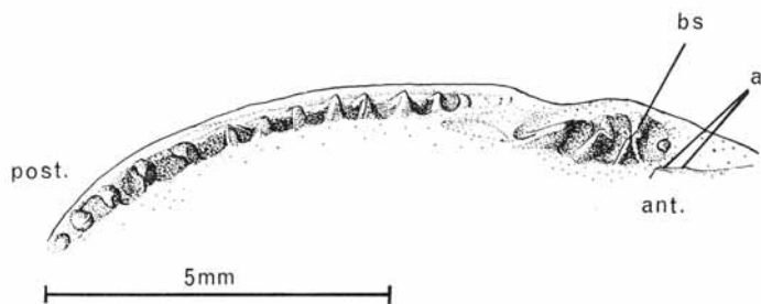
TEXT-FIG. 3. Cardiolaria beirensis . Internal mould of right valve (hinge only) showing anterior and posterior teeth and the area of resorption between them. The mould of an anterior bifid socket is indicated (bs). Specimen B.4. Llandeilo. G.R. 838495.
