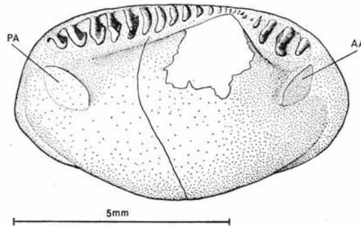
TEXT-FIG. 5. Tancrediopsis ezquerrae . Internal mould of a right valve, tilted to show the dental plate. The chevron-shaped posterior teeth decrease steadily in size towards the umbo below which they are ridge-like and low. The series is straight except just anterior of the umbo. The anterior teeth are fewer in number and show abrupt decrease in size at both ends of the series. The highest posterior tooth is equal in size to the highest anterior tooth. The junction of the two series is visible anterior of the umbo. Specimen A.12. Llandeilo. G.R. 831487.
