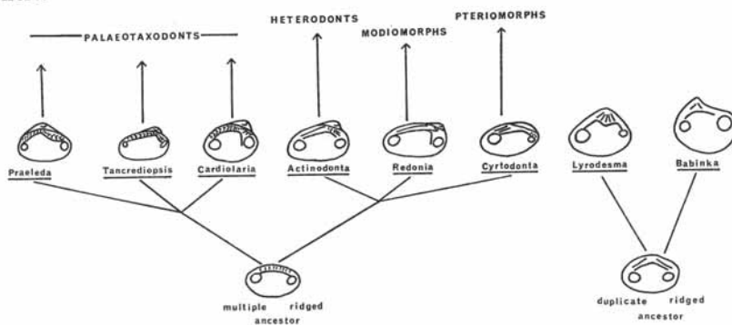
TEXT-FIG. 22. The Crozon Peninsula bivalves in a suggested Lower Palaeozoic phylogeny.
