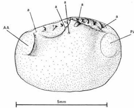
TEXT-FIG. 8. Praeleda costae . Internal mould of small left valve, anterior to left, showing early dentition and muscle scars. Specimen F.30. Llandeilo. G.R. 912441.
