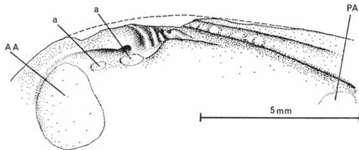
TEXT-FIG. 15. Actinodonta naranjoana . Internal mould of the hinge region of a left valve showing a dental plate possibly further developed than that shown in fig. 14. The anterior sockets (appearing as teeth) have become differentiated into three that are almost at right-angles to the dorsal margin, and one that is parallel to it. Between these and the long posterior socket is a single socket that clearly shows two fused sections. The anterior adductor and anterior accessory muscle scars are distinct. Specimen C.14.b. Llandeilo. G.R. 912441.
