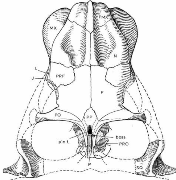
TEXT-FIG. 1. Rechinisaurus cristarhynchus , holotype. Dorsal view of skull, \times \frac{1}{4} (for abbreviations, see pp. 143-4).
