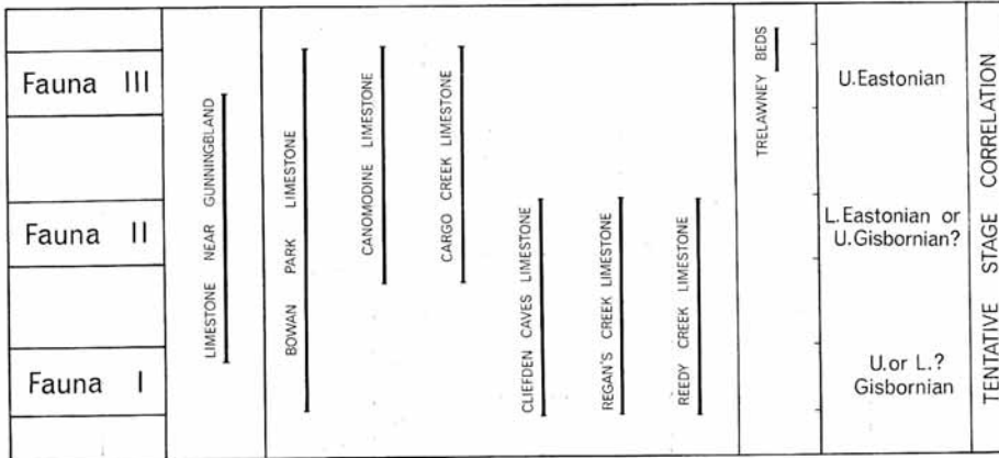
TEXT-FIG. 3. Chart showing occurrence of Faunas I-III in the Ordovician limestones of New South Wales, and their tentative correlation with the Victorian graptolite stages.
