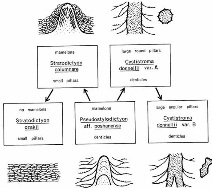
TEXT-FIG. 5. Relationships between Stratodictyon , Pseudostylocydon and Cystistroma , showing derivation of large pillars from mamelons, and small pillars from denticles. Vertical and tangential sections approximately 7 times natural scale.
