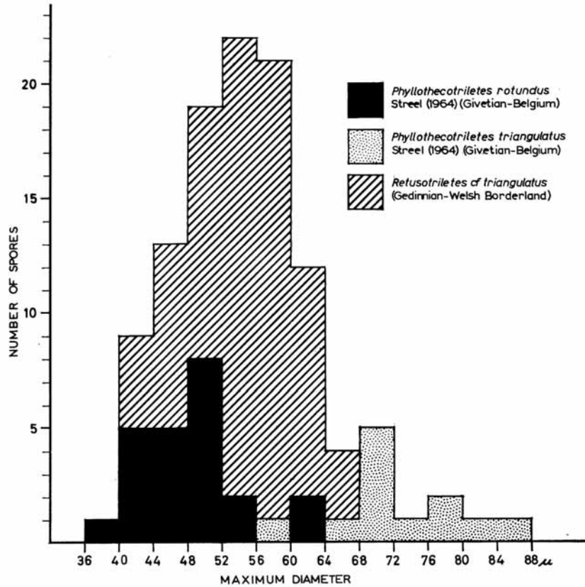
TEXT-FIG. 3. Size distribution of Retusotriletes cf. triangulatus (Stree) from the Dittonian of the Welsh Borderland compared with Stree's data from the Lower Givetian of Goé, Belgium (Stree 1964).
