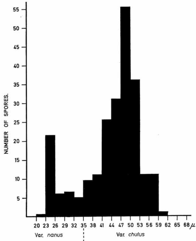
TEXT-FIG. 4. Size distribution of Archaeozonotriletes chulus (Cramer) from the Downtonian–Dittonian of the Welsh Borderland.
