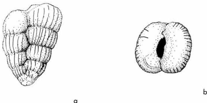
TEXT-FIG. 5. Pseudotextularia elegans (Rzehak), (a) lateral view, (b) apertural view; No. 1159, \times 100 .
