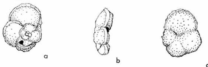
TEXT-FIG. 10. Abathomphalus intermedia (Bolli), (a) dorsal, (b) edge, and (c) ventral views; No. 1178, \times 100 .
