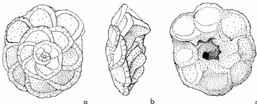
TEXT-FIG. 14. Globotruncana falsostuarti Sigal, (a) dorsal, (b) edge, and (c) ventral views; No. 1173, \times 100 .
