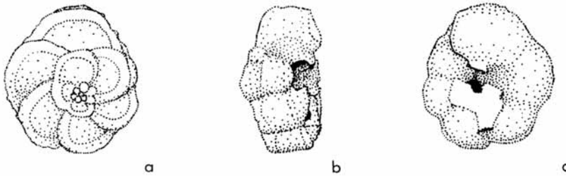
TEXT-FIG. 19. Globotruncana cf. aspera Hofker, (a) dorsal, (b) edge, and (c) ventral views; No. 1174, \times 100 .
