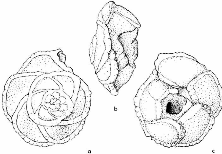
TEXT-FIG. 18. Globotruncana stuarti stuartiformis Dalbiez, (a) dorsal, (b) edge, and (c) ventral views; No. 1172, \times 100 .
