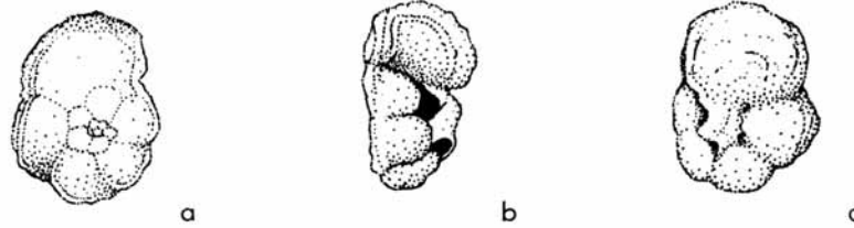
TEXT-FIG. 22. Rugoglobigerina scotti (Brönnimann), (a) dorsal, (b) edge, and (c) ventral views; No. 1180, \times 100 .
