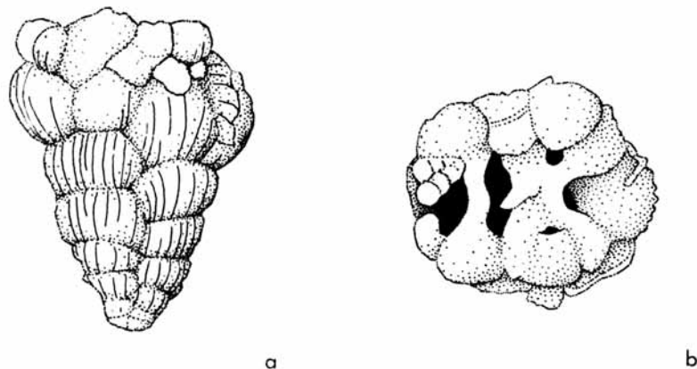
TEXT-FIG. 8. Racemiguembelina fructicosa (Egger), (a) lateral view, (b) apertural view; No. 1160, × 100.
