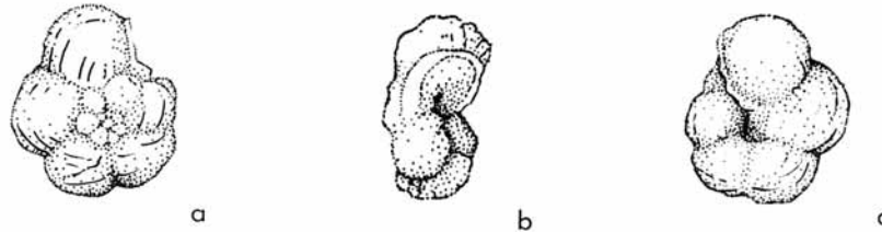
TEXT-FIG. 20. Rugoglobigerina pustulata Brönnimann, (a) dorsal, (b) edge, and (c) ventral views; No. 1181, \times 100 .
