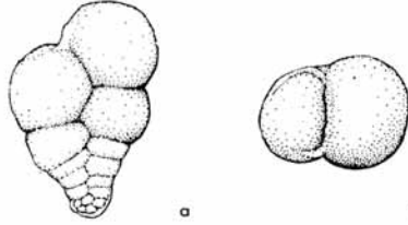
TEXT-FIG. 6. Pseudoguembelina costulata (Cushman), (a) lateral view, (b) apertural view; No. 1163, \times 100 .
