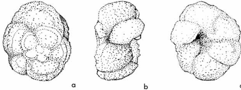
TEXT-FIG. 15. Globotruncana gansseri Bolli, (a) dorsal, (b) edge, and (c) ventral views; No. 1175, \times 100 .
