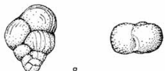
TEXT-FIG. 2. Heterohelix striata (Ehrenberg), (a) lateral view, (b) apertural view; No. 1164, \times 100 .
