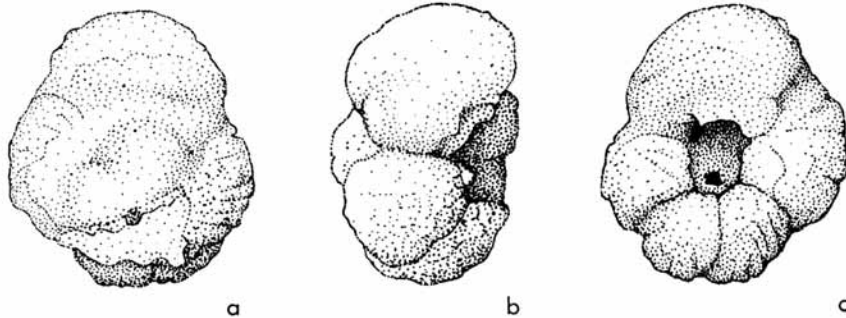
TEXT-FIG. 21. Rugoglobigerina rotundata Brönnimann, (a) dorsal, (b) edge, and (c) ventral views; No. 1179, × 100.
