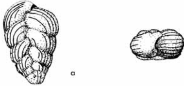
TEXT-FIG. 1. Heterohelix globulosa (Ehrenberg), b (a) lateral view, (b) apertural view; No. 1165, \times 100 .
