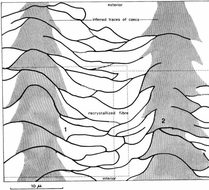
TEXT-FIG. 2. Tracing of montage showing the disposition of recrystallized secondary fibres in a transverse section of a pedicle valve of Kotujella calva Andreeva in relation to two adjacent canals inferred to have accommodated caeca; the areas occupied by figs. 5 and 6 of Plate 92 are indicated as 1 and 2 respectively.
