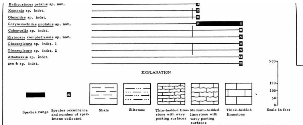
TEXT-FIG. 1. Chart showing the local range of trilobite species in the Pioche Shale, Campbell Ranch Section, East-Central Nevada, U.S.A.
