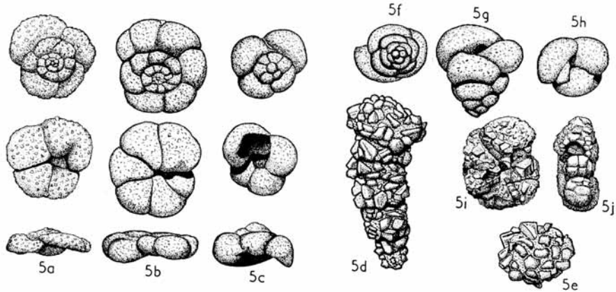
TEXT-FIG. 5. Trochammina , Reophax , Haplophragmoides , and Eggerella ? 5a, Dorsal, ventral, and lateral views of Trochammina squamata , P. 43978, \times 41 , baylei zone, Black Head, near Osmington Mills, Grid ref. 30/727818. 5b, Dorsal, ventral, and lateral views of T. cf. nitida , P. 43979, \times 72.5 , Crushed Ammonoid Shales, rotunda zone, Hounstout, Grid ref. 30/947773. 5c, Dorsal, lateral, and ventral views of T. globigeriniformis , P. 43980, \times 102.5 , pectinatus zone, Freshwater Steps, Grid ref. 30/942773. 5d, e, Lateral and terminal views of Reophax hounstoutensis sp. nov., holotype, P. 43984, \times 36 . 5f, g, h, Lateral, initial, and terminal views of Eggerella? meentzeni , P. 43981, \times 82 , mutabilis zone, Black Head, near Osmington Mills, Grid ref. 30/727818. 5i, j, Lateral and peripheral views of Haplophragmoides haesleri sp. nov., holotype, P. 43985, \times 43.5 .
