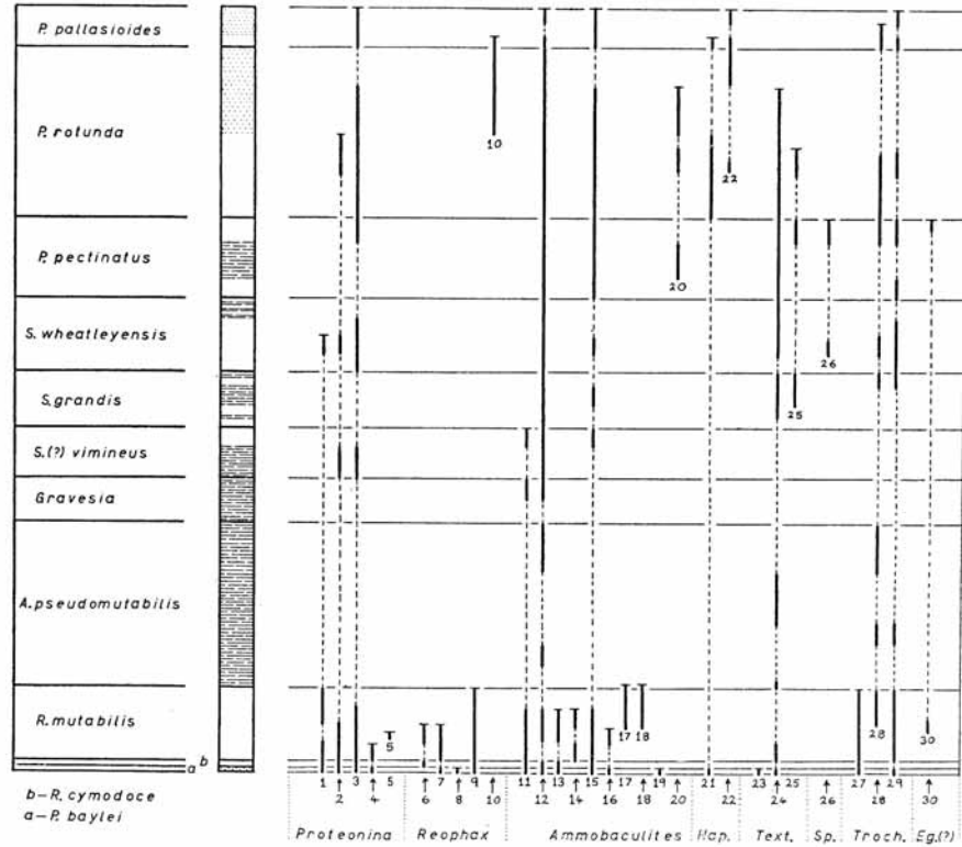
TEXT-FIG. 2. Table showing ranges of arenaceous foraminifera in the Kimeridgian.
