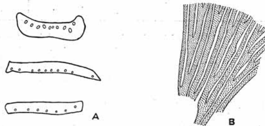
TEXT-FIG. 3. Calcifolium bruntonense sp. nov. (A) Transverse and tangential sections of branch fragments, \times 30 , PF 621; (B) detail of dichotomously branching canals in a lateral branch, longitudinal section \times 50 , PF 622.
