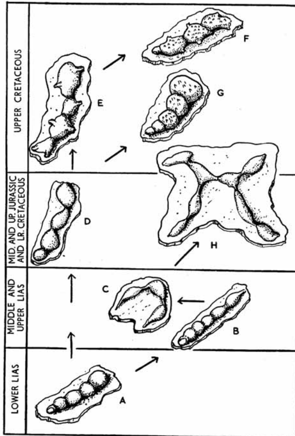
TEXT-FIG. 2. Outline of evolution of Bullopورا .
